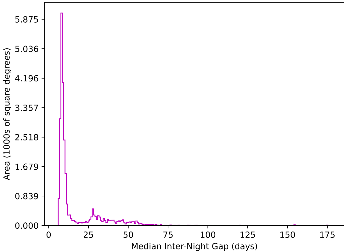
weather_cloudso0v3.5_10yrs All sky z band: Median Inter-Night Gap
