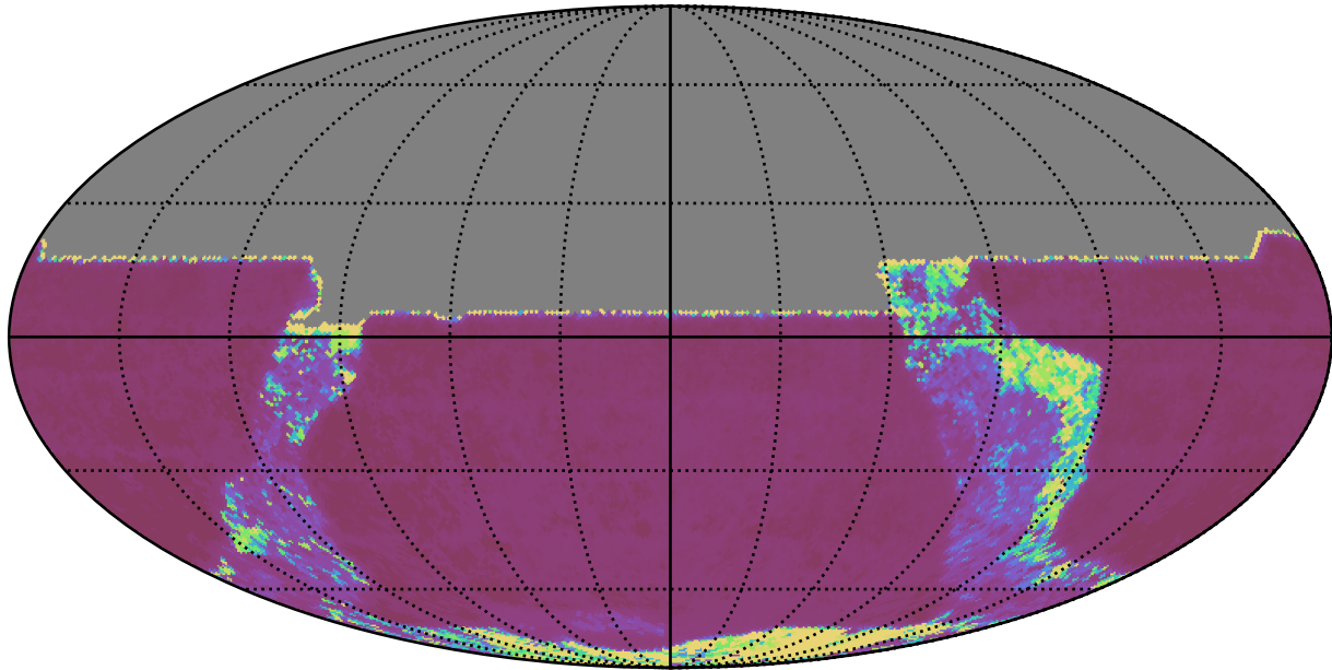
weather_cloudso0v3.5_10yrs All sky y band: Median Inter-Night Gap
