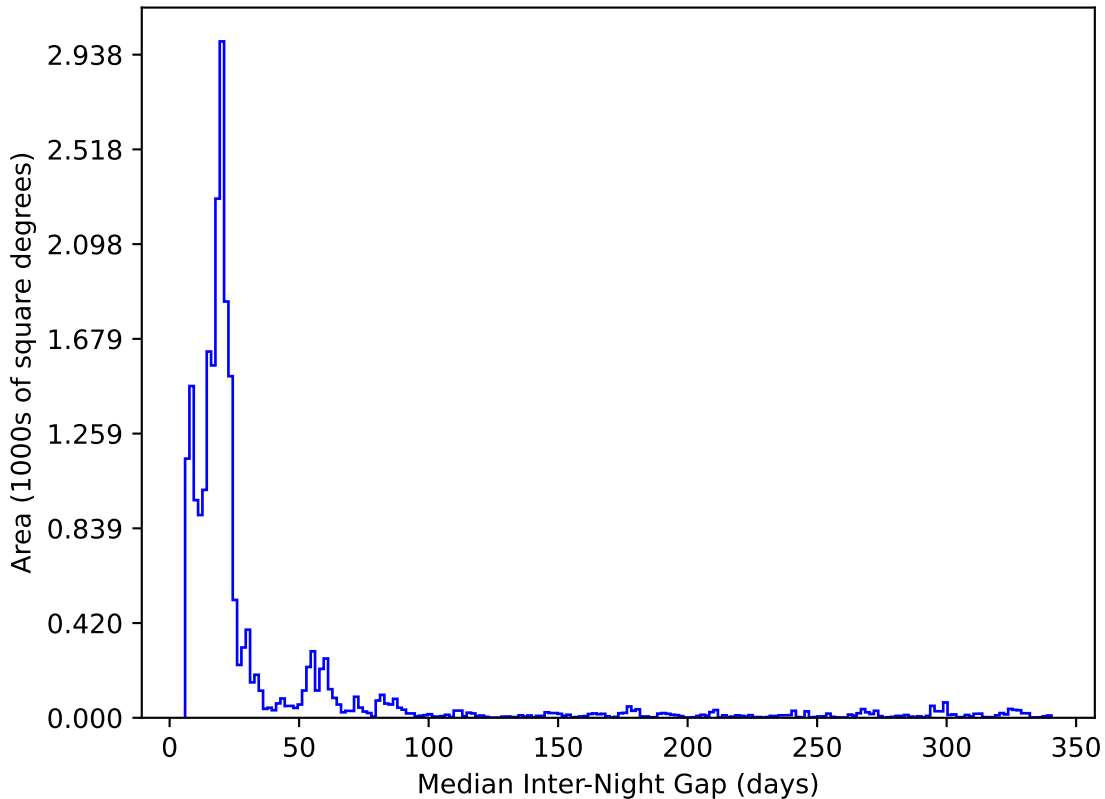
weather_cloudso0v3.5_10yrs All sky y band: Median Inter-Night Gap
