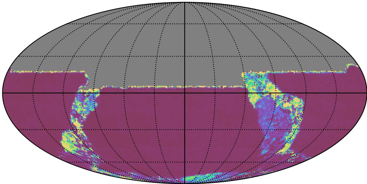
weather_cloudso0v3.5_10yrs All sky u band: Median Inter-Night Gap
