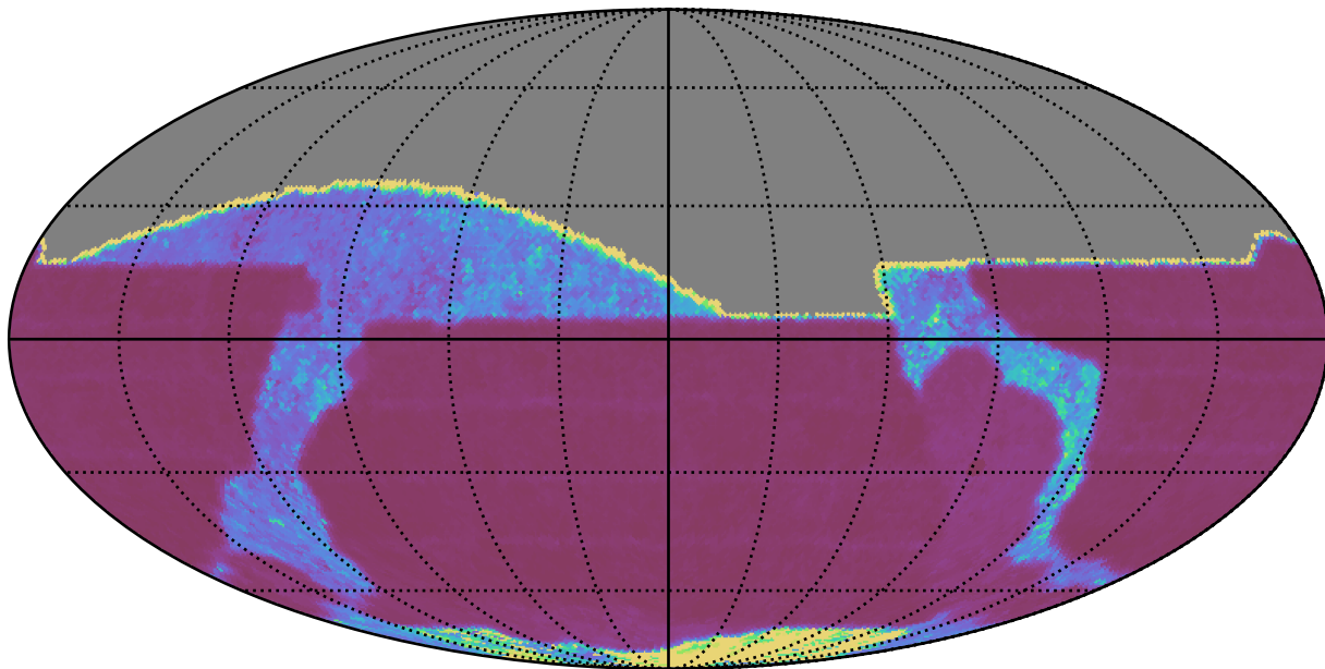
weather_cloudso0v3.5_10yrs All sky i band: Median Inter-Night Gap
