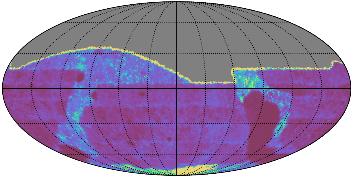
weather_cloudso0v3.5_10yrs All sky g band: Median Inter-Night Gap
