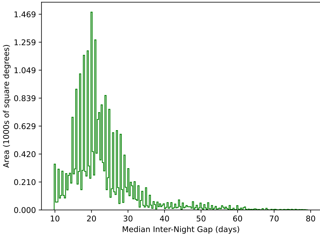
weather_cloudso0v3.5_10yrs All sky g band: Median Inter-Night Gap
