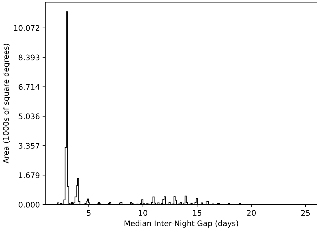
weather_cloudso0v3.5_10yrs All sky all bands: Median Inter-Night Gap
