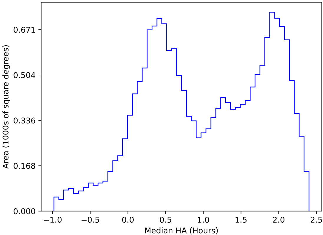
weather_cloudso0v3.5_10yrs WFD z band: Median HA
