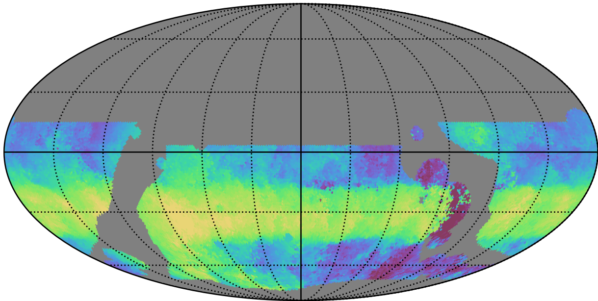
weather_cloudso0v3.5_10yrs WFD u band: Median HA
