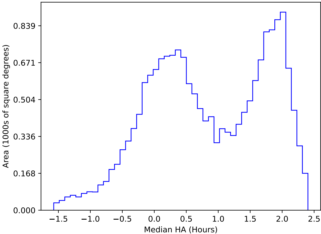
weather_cloudso0v3.5_10yrs WFD u band: Median HA
