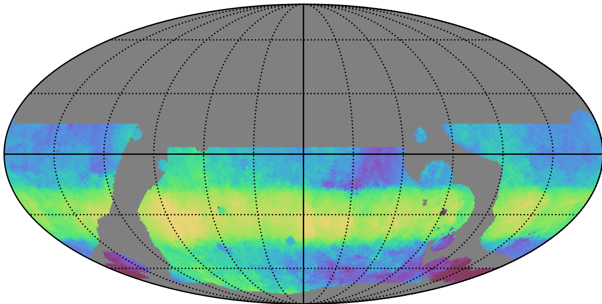
weather_cloudso0v3.5_10yrs WFD r band: Median HA
