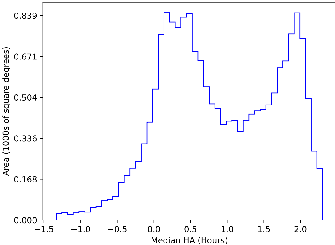
weather_cloudso0v3.5_10yrs WFD r band: Median HA
