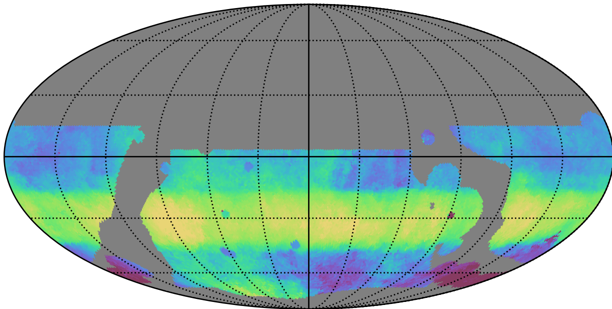
weather_cloudso0v3.5_10yrs WFD i band: Median HA
