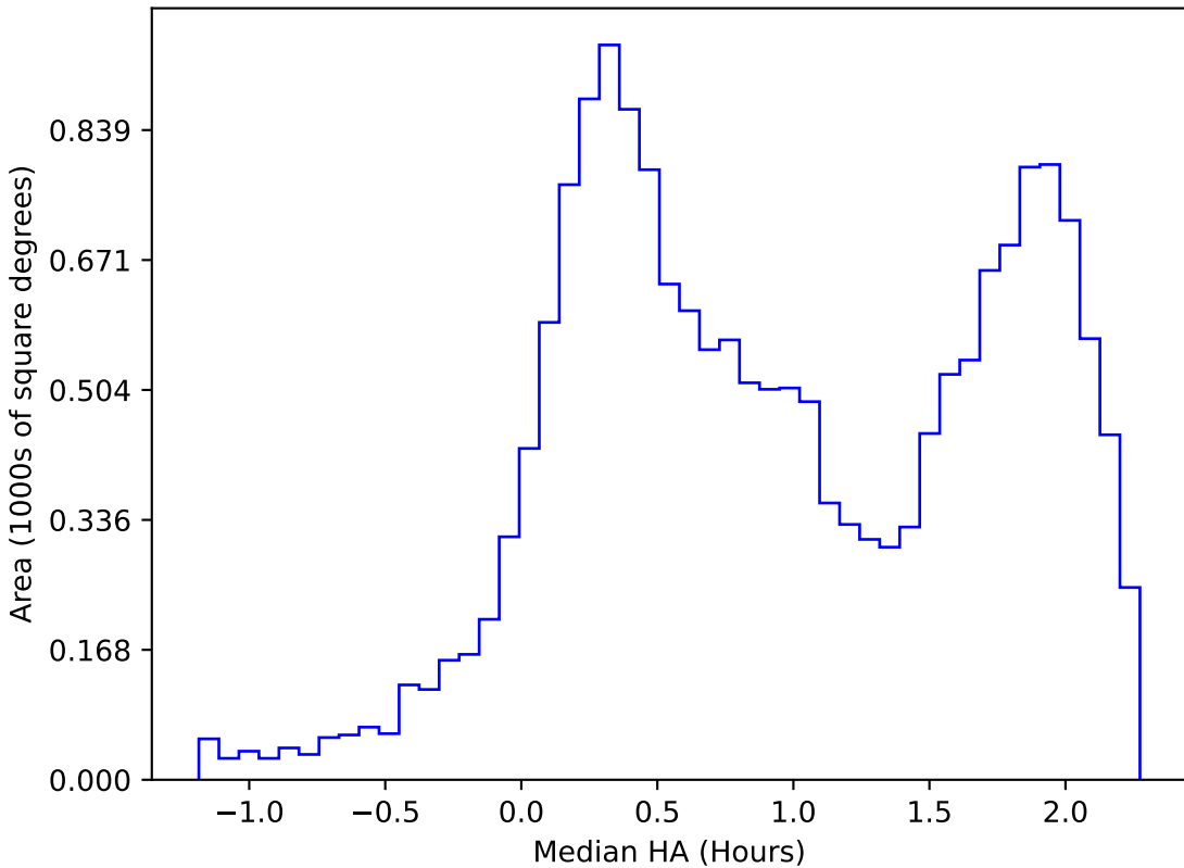
weather_cloudso0v3.5_10yrs WFD i band: Median HA
