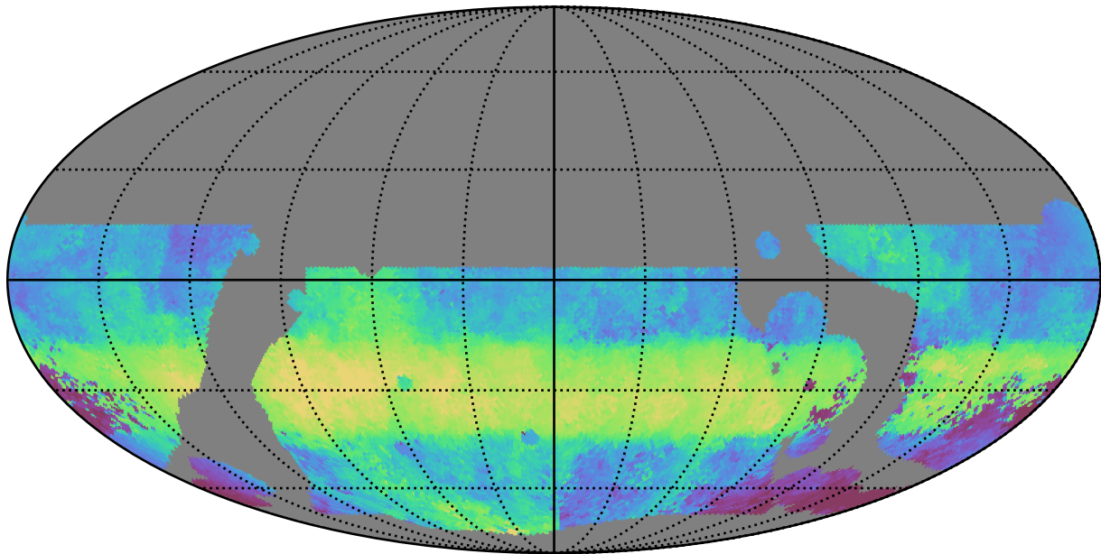
weather_cloudso0v3.5_10yrs WFD g band: Median HA
