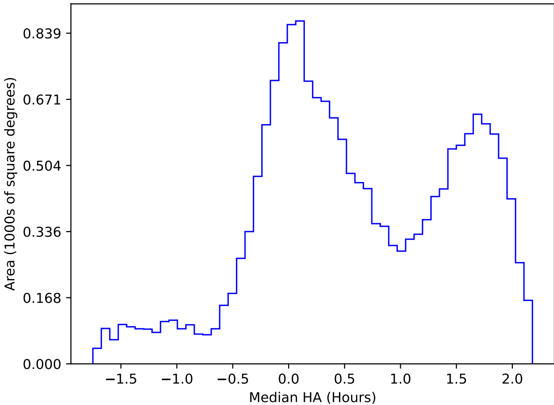
weather_cloudso0v3.5_10yrs WFD g band: Median HA
