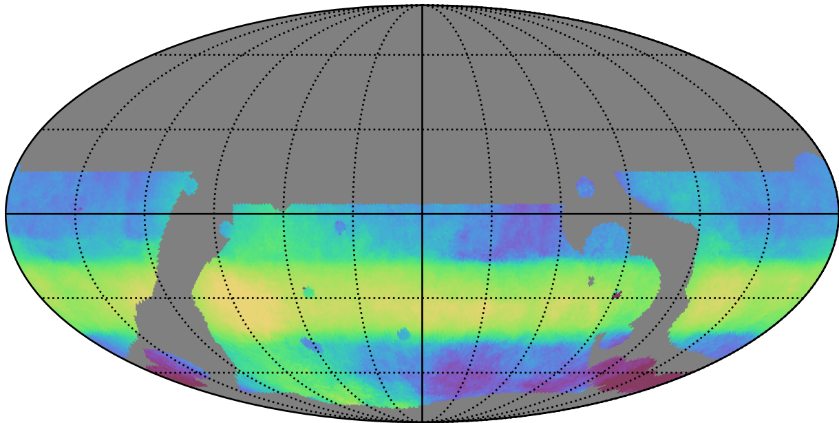
weather_cloudso0v3.5_10yrs WFD all bands: Median HA
