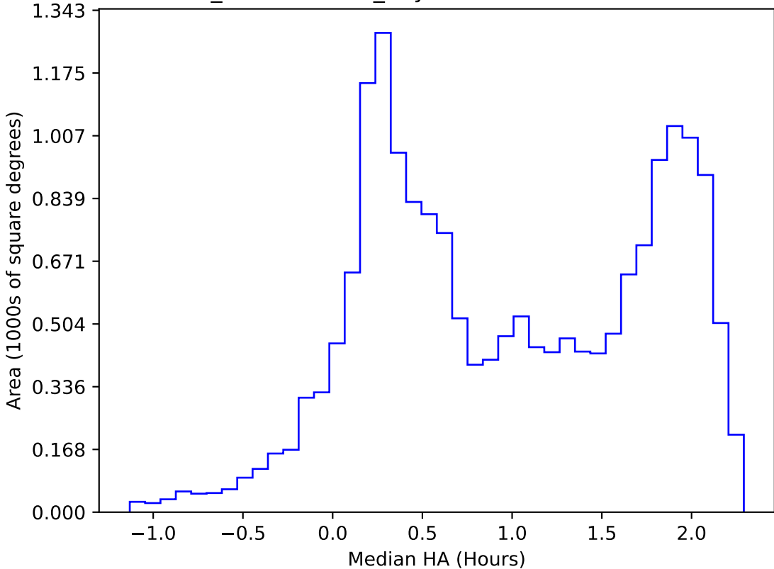
weather_cloudso0v3.5_10yrs WFD all bands: Median HA
