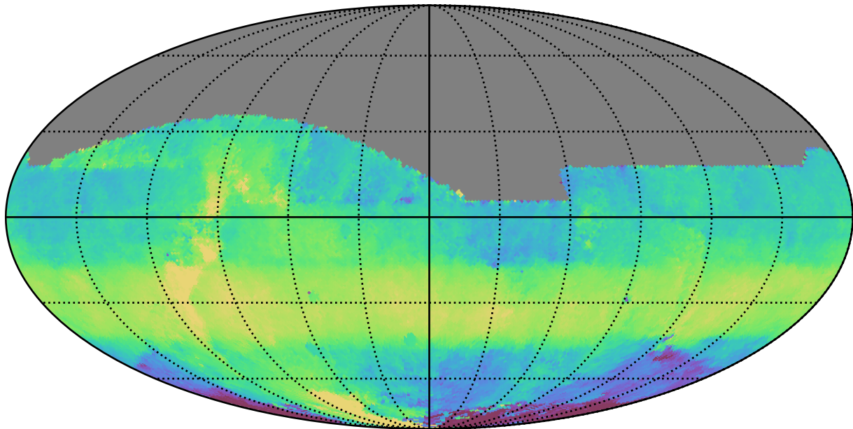
weather_cloudso0v3.5_10yrs All sky z band: Median HA
