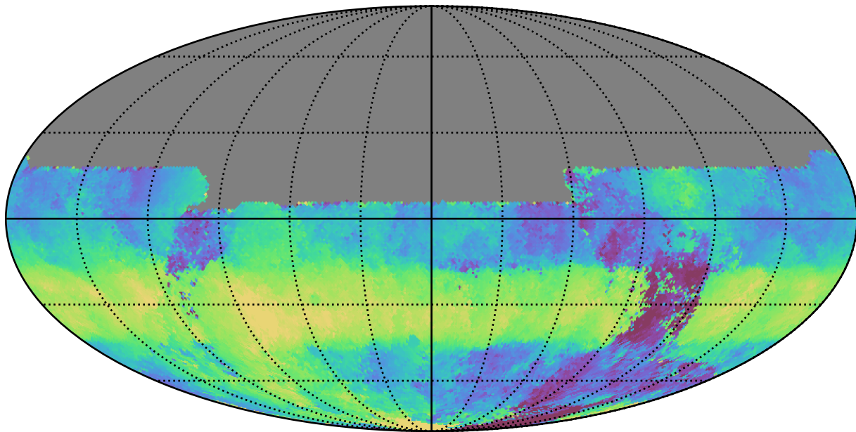
weather_cloudso0v3.5_10yrs All sky u band: Median HA
