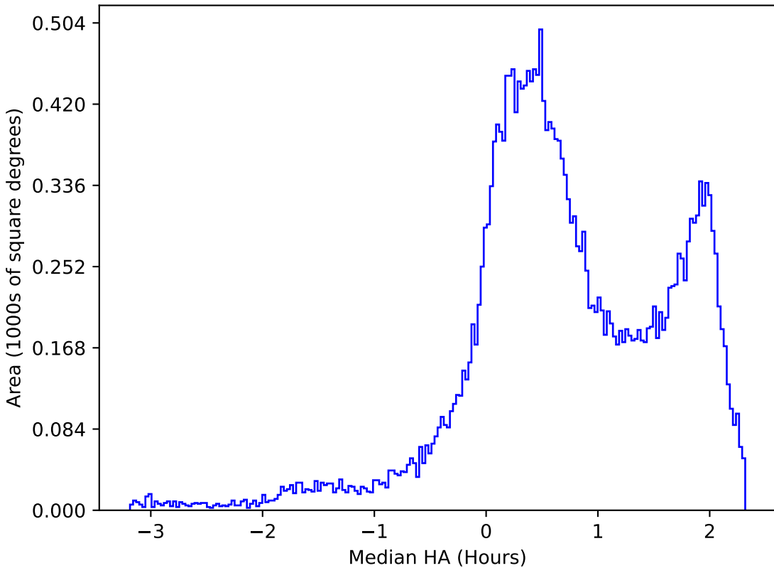
weather_cloudso0v3.5_10yrs All sky r band: Median HA
