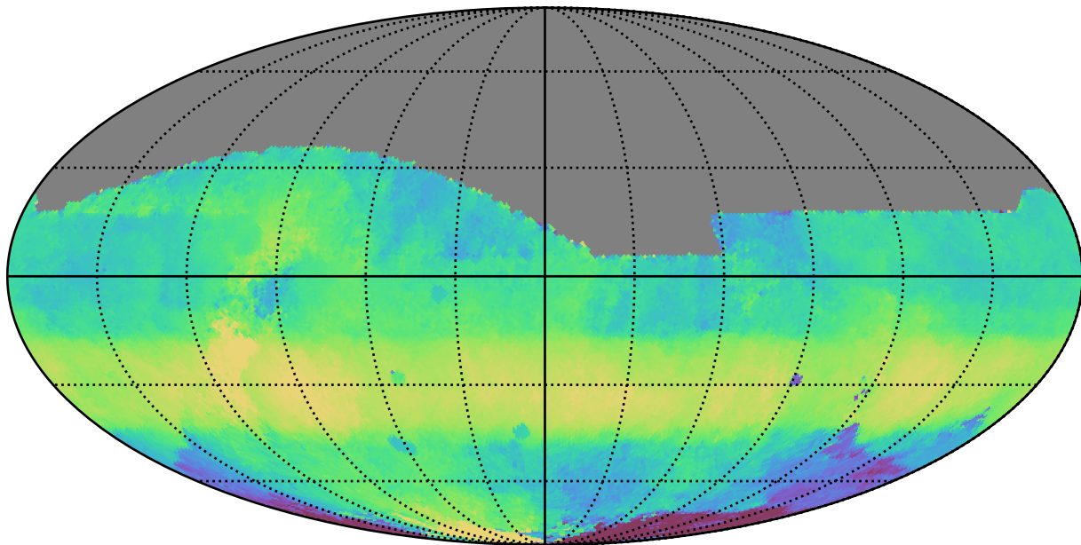
weather_cloudso0v3.5_10yrs All sky i band: Median HA
