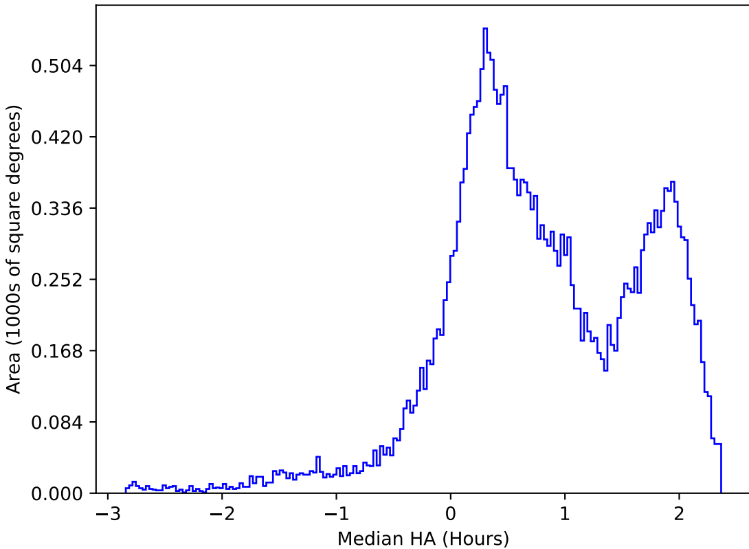
weather_cloudso0v3.5_10yrs All sky i band: Median HA
