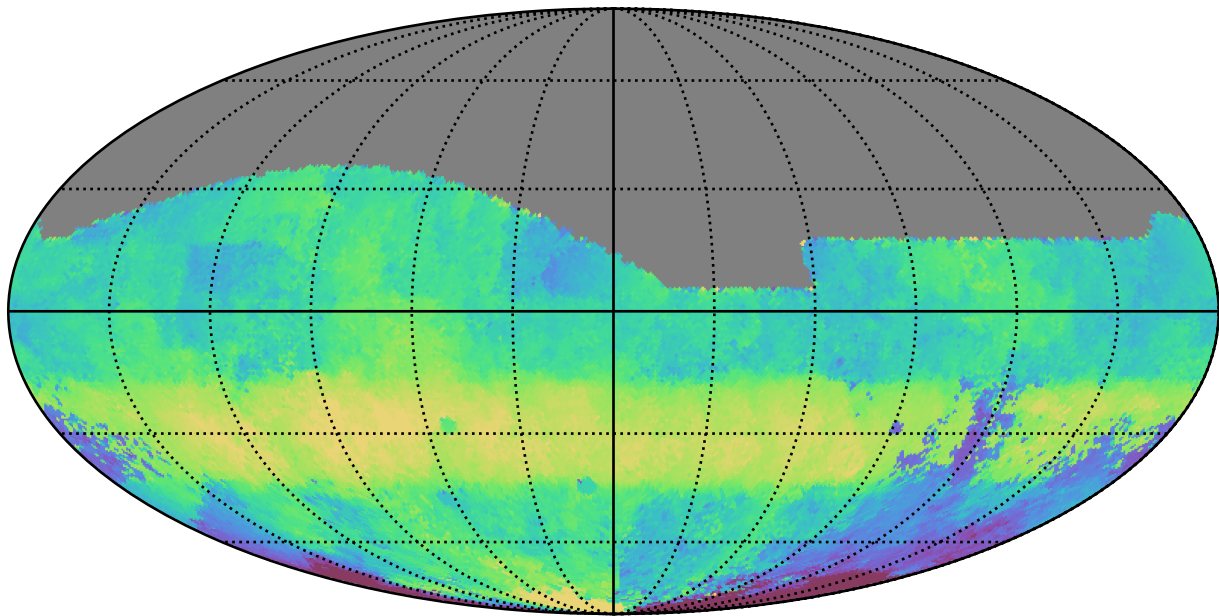
weather_cloudso0v3.5_10yrs All sky g band: Median HA
