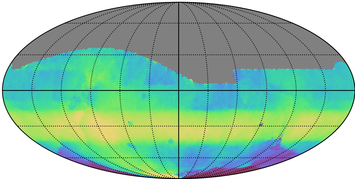
weather_cloudso0v3.5_10yrs All sky all bands: Median HA
