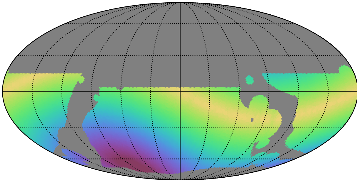
weather_cloudso0v3.5_10yrs WFD z band: Max solarElong
