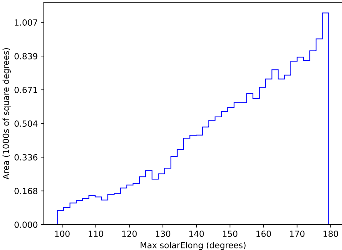
weather_cloudso0v3.5_10yrs WFD z band: Max solarElong
