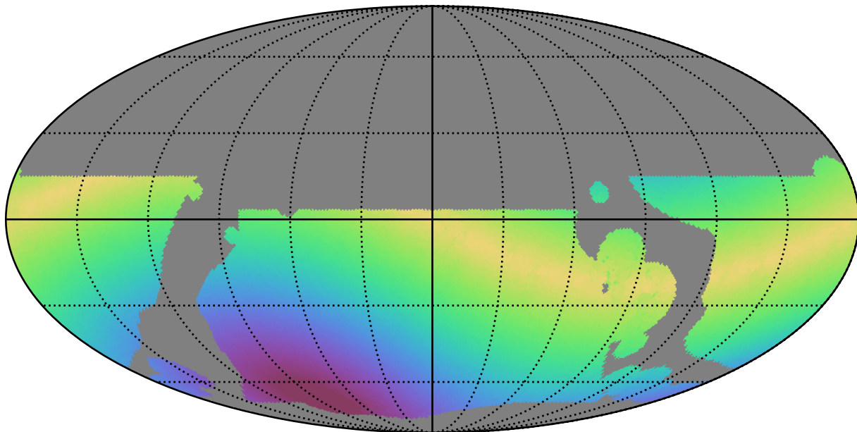
weather_cloudso0v3.5_10yrs WFD y band: Max solarElong
