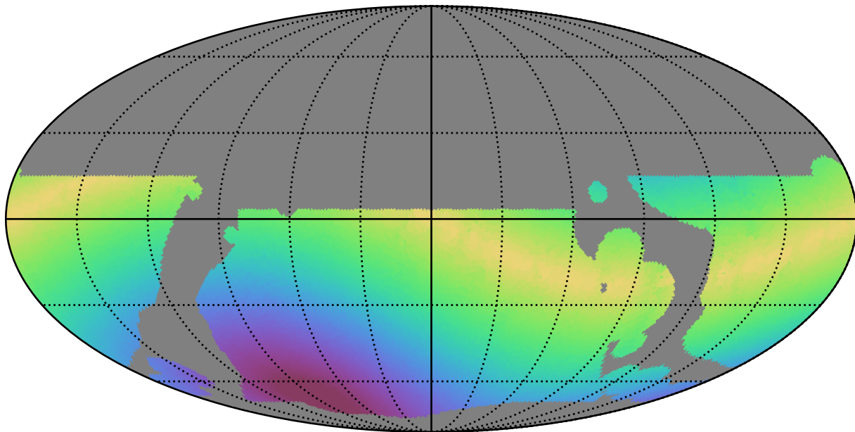
weather_cloudso0v3.5_10yrs WFD u band: Max solarElong
