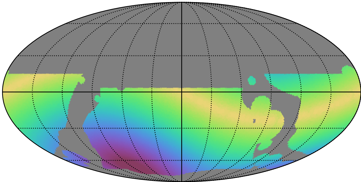
weather_cloudso0v3.5_10yrs WFD r band: Max solarElong
