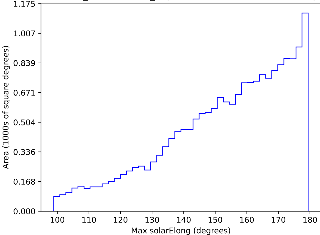
weather_cloudso0v3.5_10yrs WFD r band: Max solarElong
