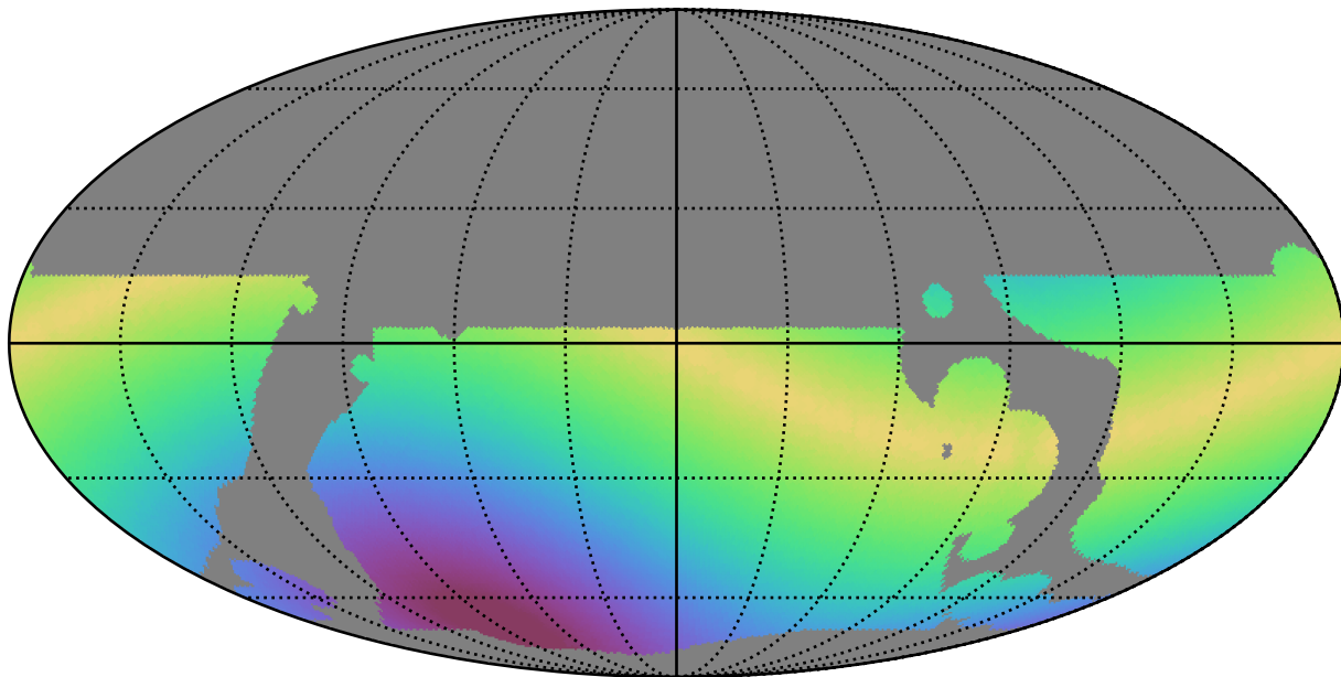
weather_cloudso0v3.5_10yrs WFD i band: Max solarElong
