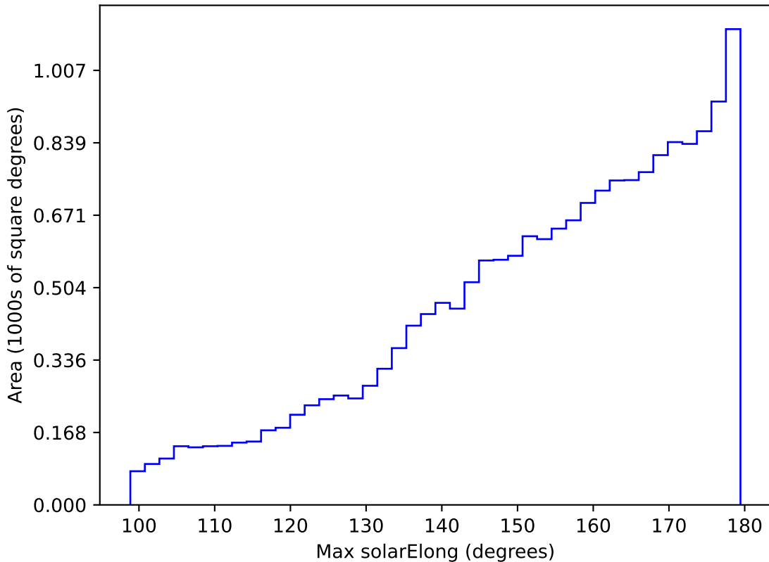
weather_cloudso0v3.5_10yrs WFD i band: Max solarElong
