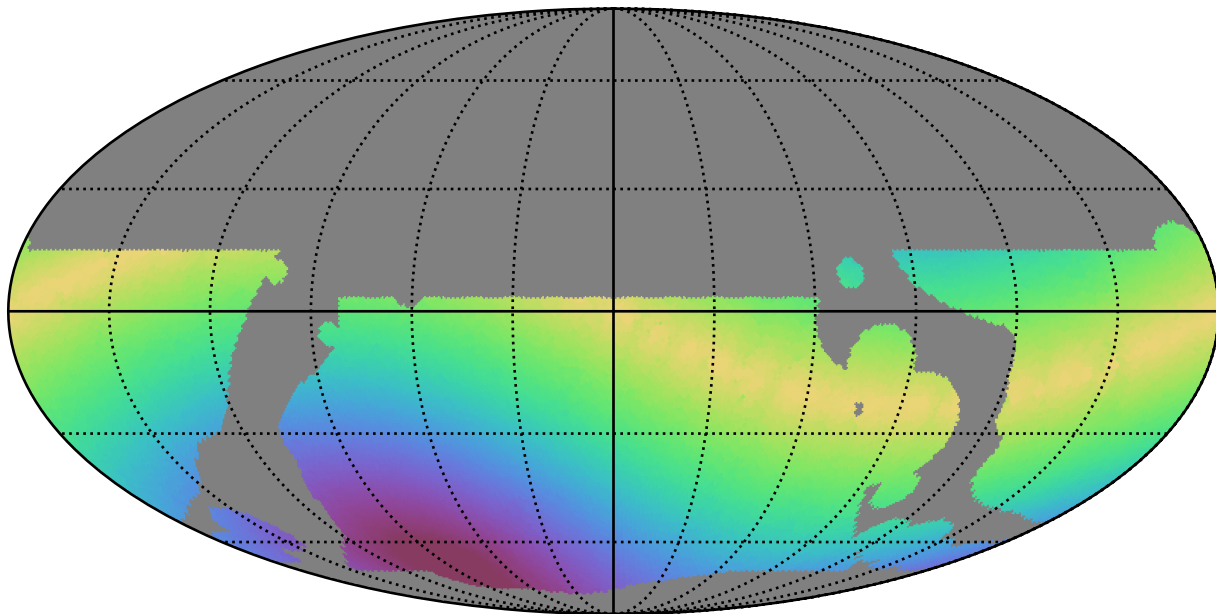
weather_cloudso0v3.5_10yrs WFD g band: Max solarElong
