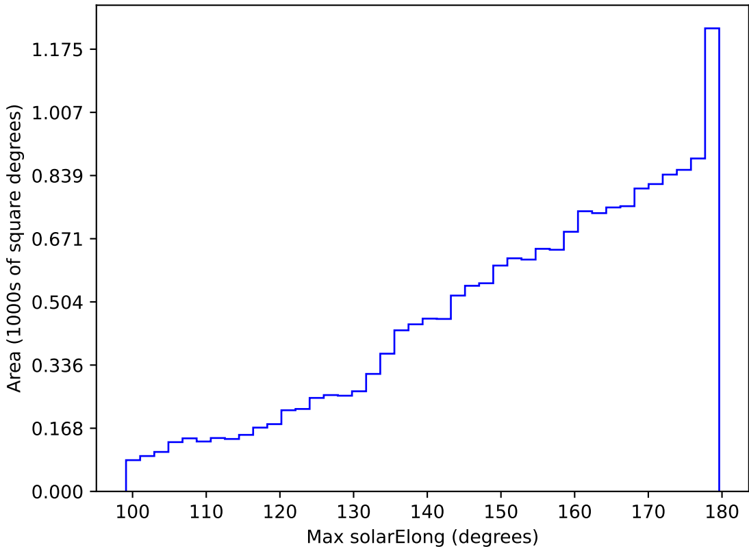
weather_cloudso0v3.5_10yrs WFD all bands: Max solarElong
