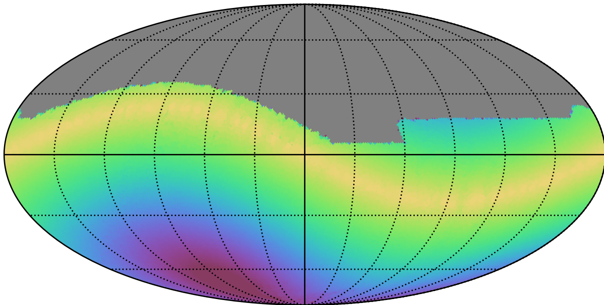
weather_cloudso0v3.5_10yrs All sky z band: Max solarElong
