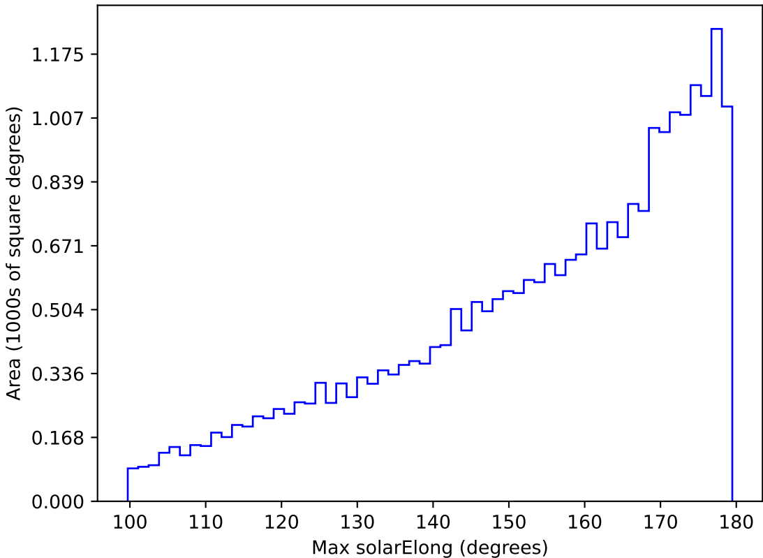
weather_cloudso0v3.5_10yrs All sky z band: Max solarElong
