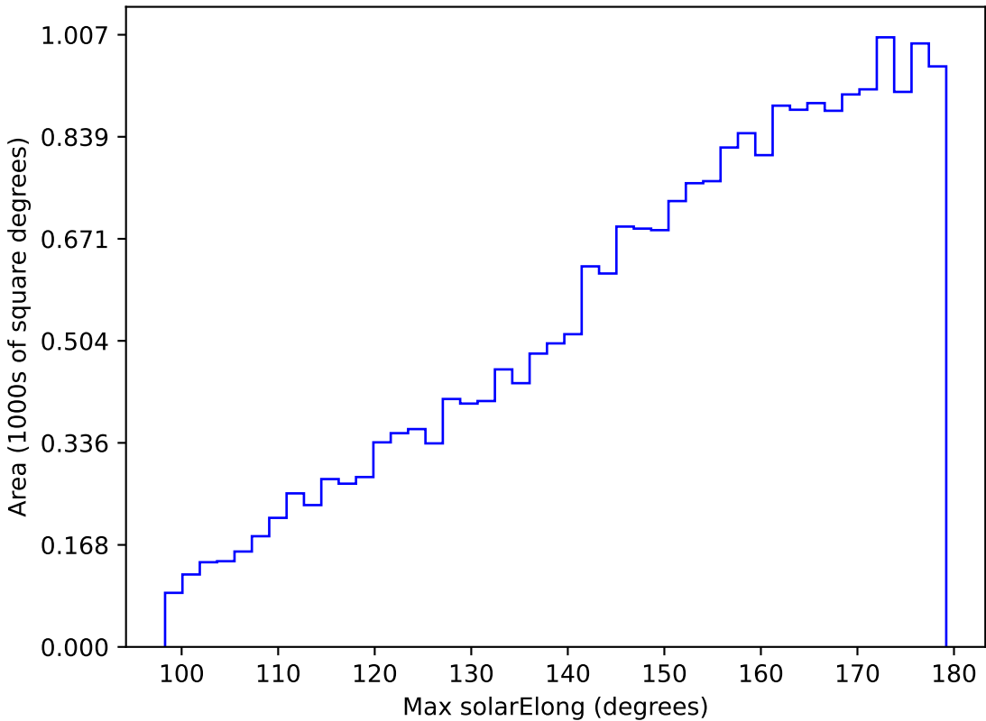
weather_cloudso0v3.5_10yrs All sky y band: Max solarElong
