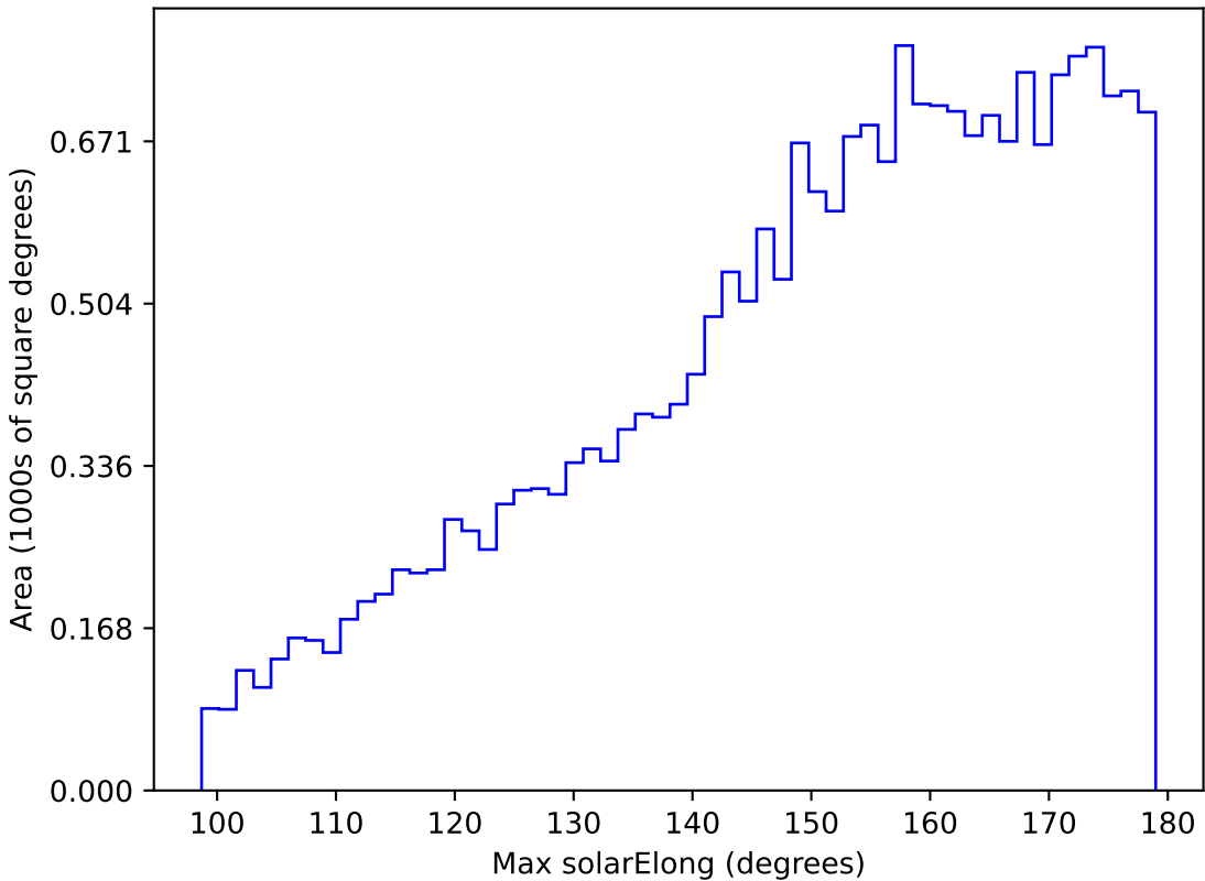
weather_cloudso0v3.5_10yrs All sky u band: Max solarElong
