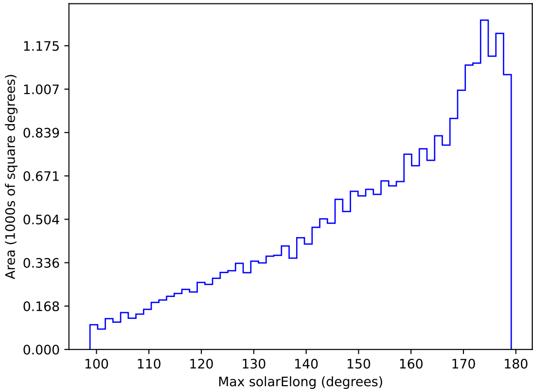
weather_cloudso0v3.5_10yrs All sky g band: Max solarElong
