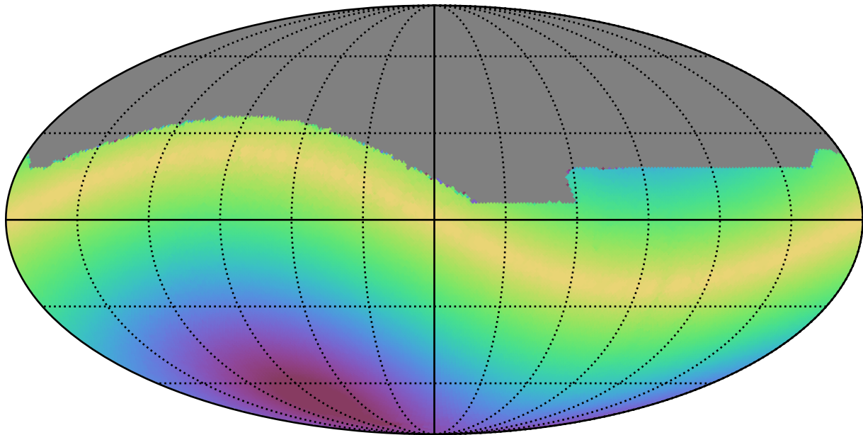
weather_cloudso0v3.5_10yrs All sky all bands: Max solarElong
