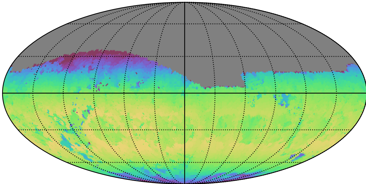
weather_cloudso0v3.5_10yrs Yr 1 z band: Max skyBrightness
