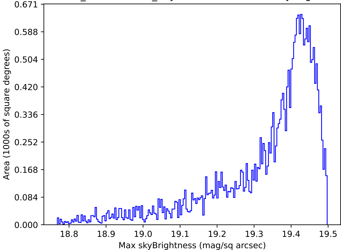
weather_cloudso0v3.5_10yrs Yr 1 z band: Max skyBrightness
