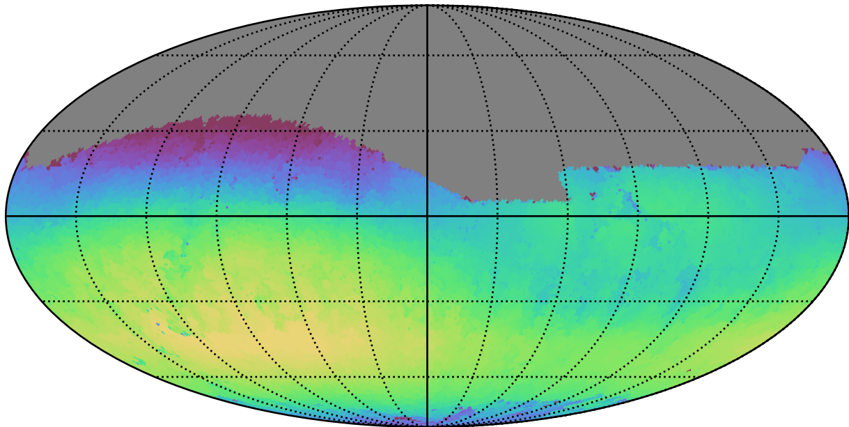
weather_cloudso0v3.5_10yrs Yr 1 r band: Max skyBrightness
