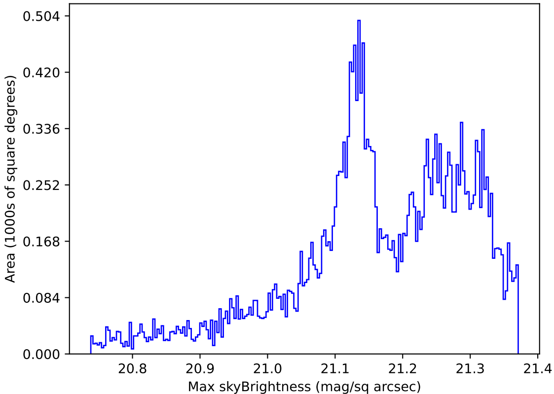
weather_cloudso0v3.5_10yrs Yr 1 r band: Max skyBrightness
