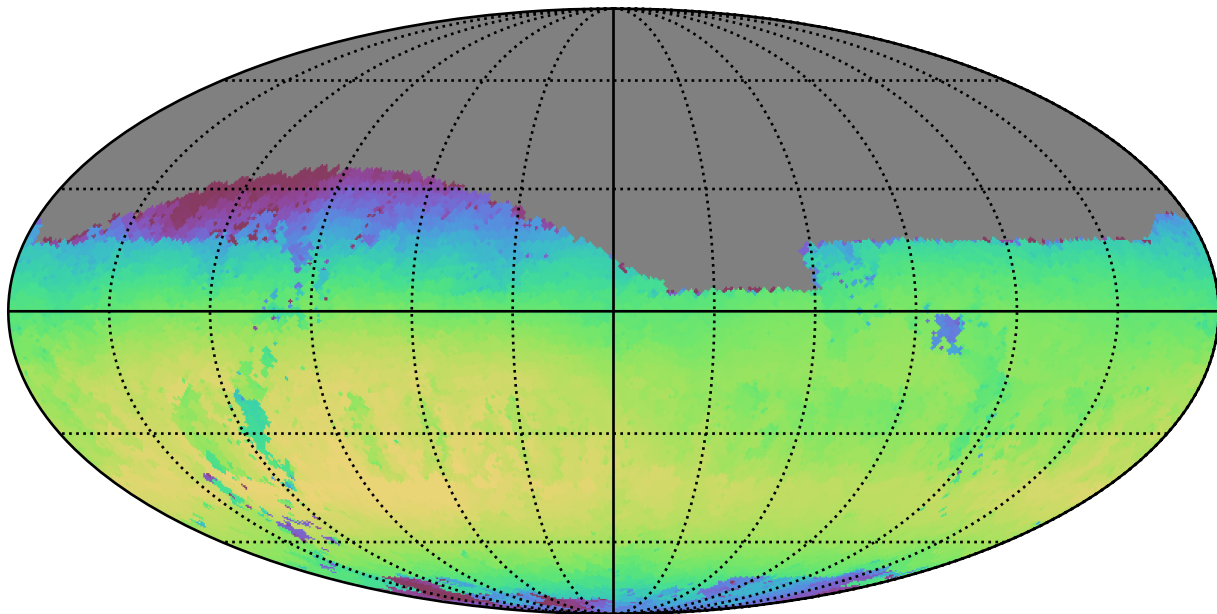
weather_cloudso0v3.5_10yrs Yr 1 i band: Max skyBrightness
