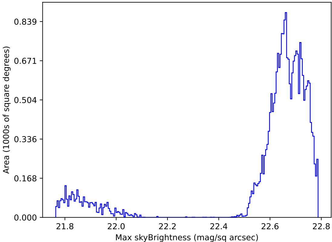
weather_cloudso0v3.5_10yrs Yr 1 all bands: Max skyBrightness
