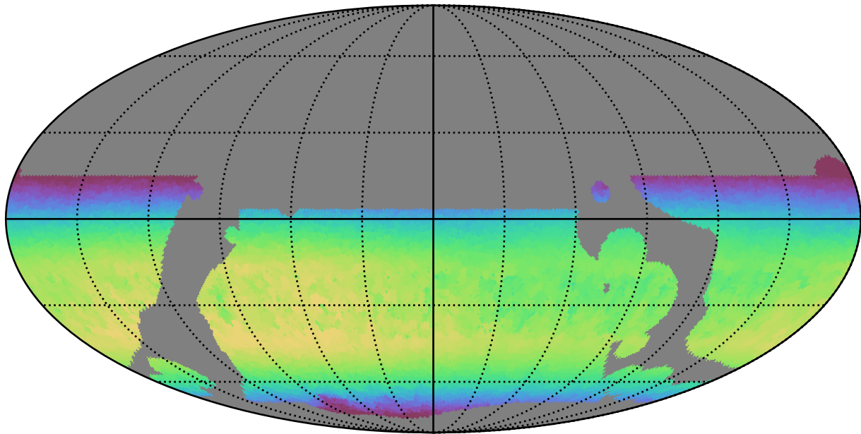
weather_cloudso0v3.5_10yrs WFD z band: Max skyBrightness
