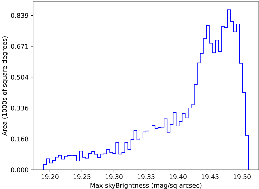
weather_cloudso0v3.5_10yrs WFD z band: Max skyBrightness
